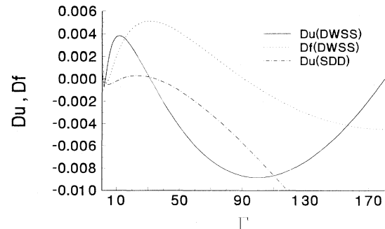
FIG. 2. Comparison of different fits for the OCP excess energies: Du(\text{DWSS}) = u_0^{\text{OIIVH}} - u_0^{\text{DWSS}} , Df(\text{DWSS}) = f_0^{\text{OIIVH}} - f_0^{\text{DWSS}} , and Du(\text{SDD}) = u_0^{\text{OIIVH}} - u_0^{\text{SDD}} . See the text.
