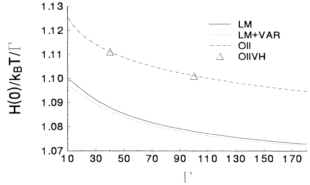
FIG. 1. Consistency with respect to the zero-separation sum rule. h_0 = H(0)/(k_B T / \Gamma) . OII [Eq. (12)], LM [Eqs. (9) and (14)], LM+VAR [Eqs. (8), (11), and (18)], and OIIVH [Eq. (8) and the fit of [2]]. LM+VAR represents the present results for the deviations from linear mixing, while OIIVH are the corresponding results from Ref. [2] (see the text).
